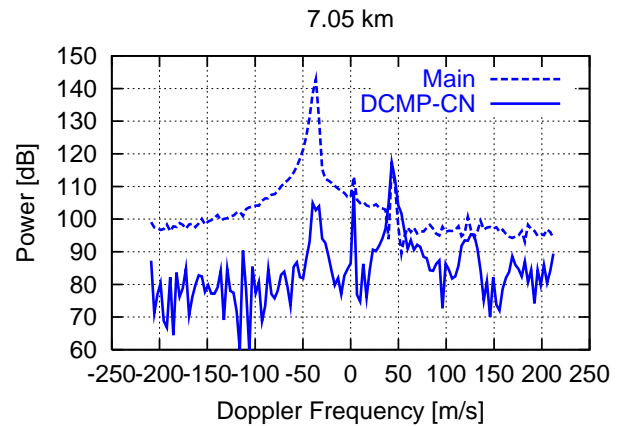
Fig. 8. Same as Fig.7, but for a sampling interval of 7.6ms.
