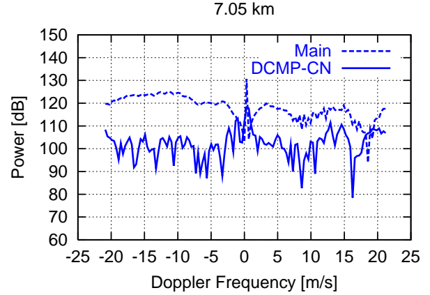
Fig. 7. Example of the Doppler echo power spectrum with strong aircraft echo at a sampling interval of 76ms from raw main beam data (dashed) and with proposed DCMP-CN algorithm (solid). The y-axis indicates received power in arbitrary units.
