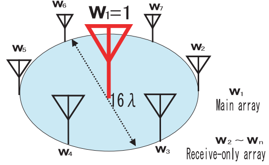
Fig. 1. Configuration of a high-gain antenna with a peripheral receive-only sub-array.
