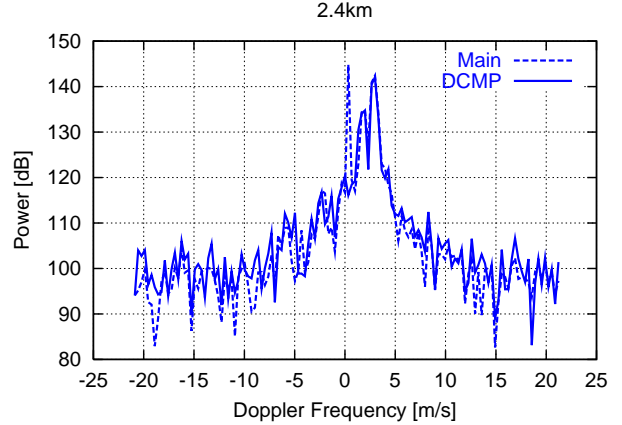
Fig. 4. Doppler echo power spectrum at 2.4km range raw main beam data (dashed) and processed with conventional DCMP algorithm (solid). The y-axis indicates received power in arbitrary units.
