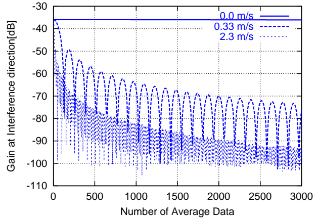
Fig. 9. Gain in direction of interferer for monochromatic signals with different Doppler velocities.
